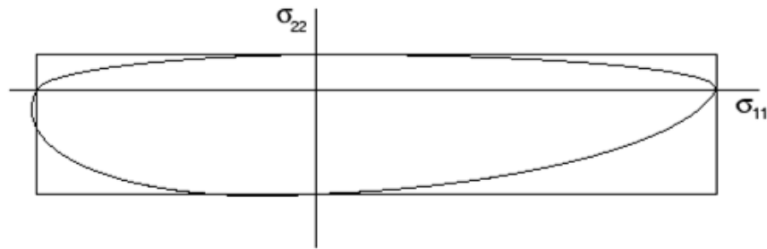
Figure 1.6.1: Tsai-Hill piecewise-continuous failure surface
