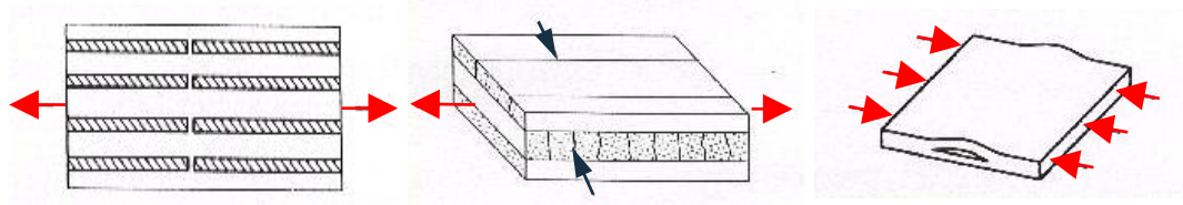
Figure 1.2.1: (L-R) Fibre, matrix and delamination failure
