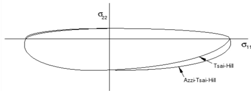
Figure 1.9.1: Azzi-Tsai-Hill piecewise-continuous failure surface
